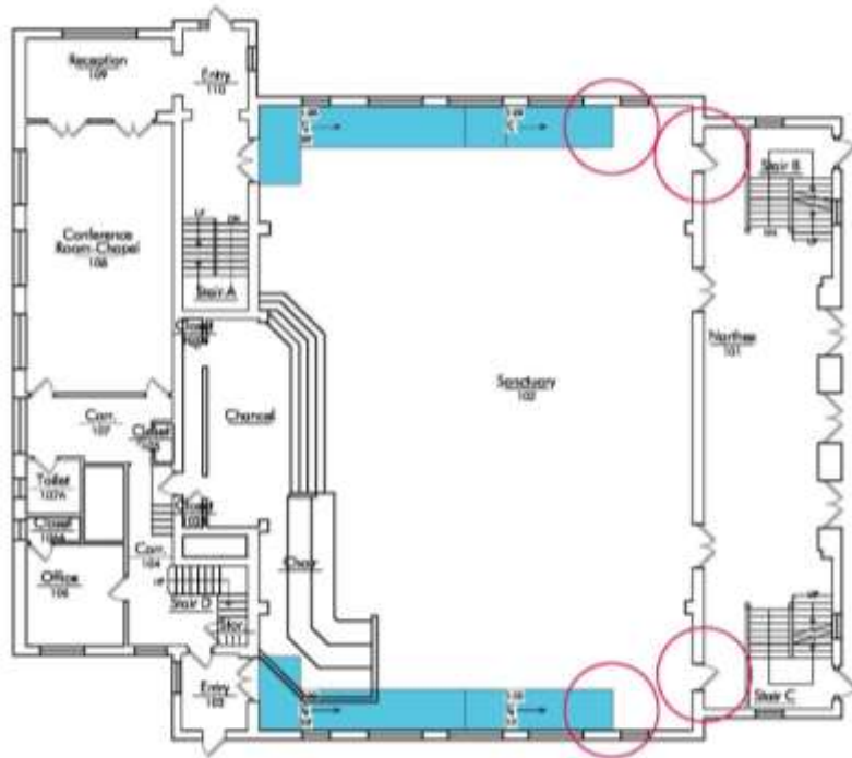
Sanctuary without raked floor
