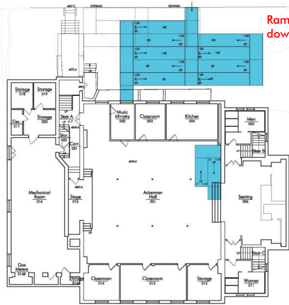
Lower Level Accessibility – Ramped
