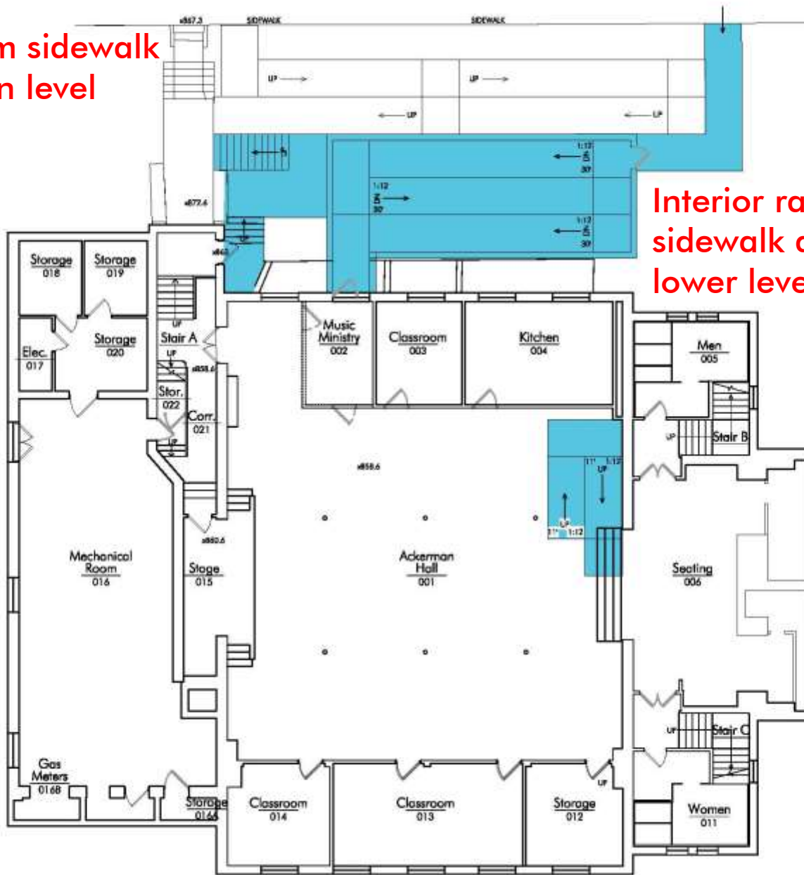
Lower and Main Level Accessibility – Ramped (interior and exterior)
