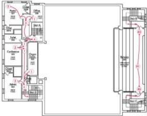
UPPER LEVEL EGRESS PLAN
