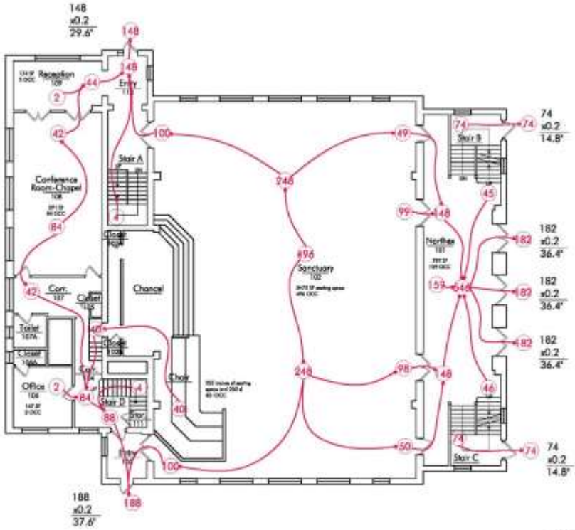
MAIN LEVEL EGRESS PLAN
