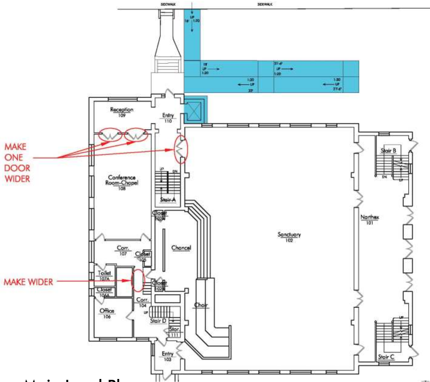
Main Level Plan Option 3: Full Access with Elevator
