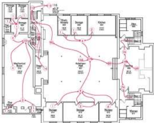
LOWER LEVEL EGRESS PLAN
